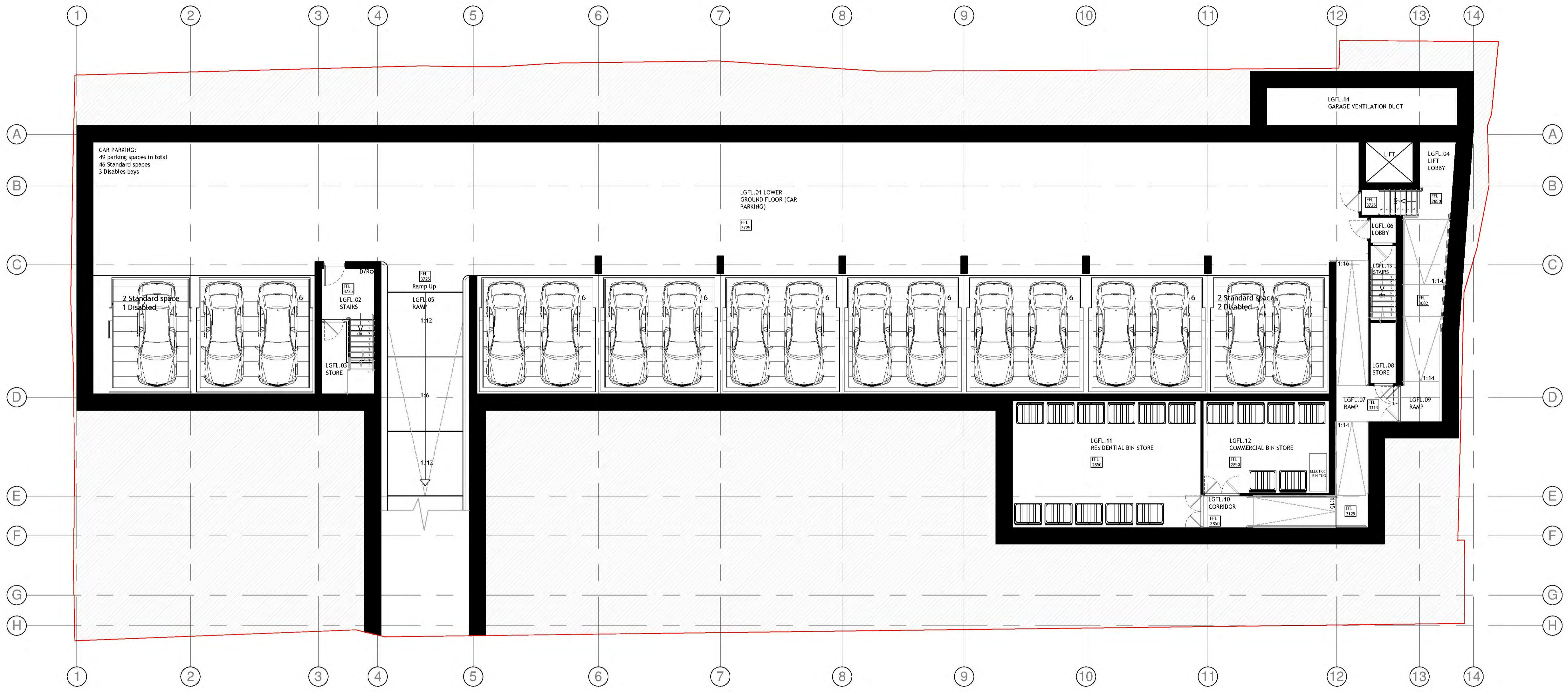
LOWER GROUND FLOOR Scale 1:100
